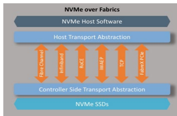
Figure 1 -- NVME-oF topology.
