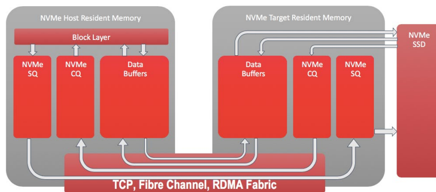
Figure 2 -- NVMe-oF with Current Fabrics
