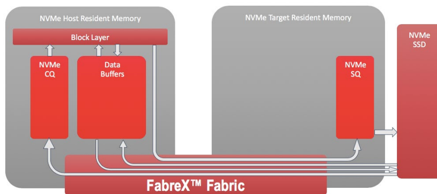
Figure 3 -- NVMe-oF GigaIO FabreX Implementation
