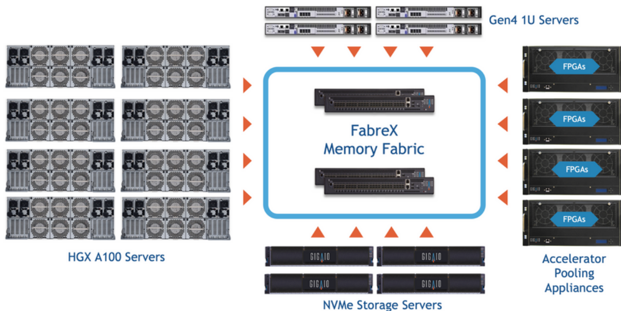
SDSC GigalO Composable Disaggregated System Configuration
