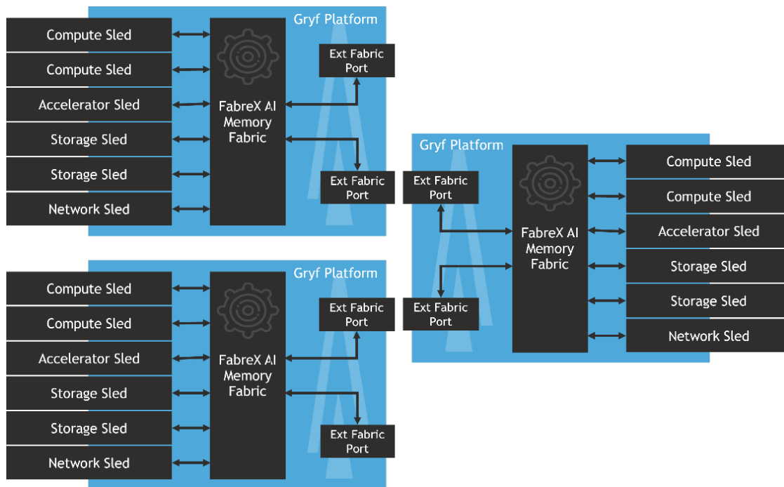
Interconnect up to five Gryfs across FabreX, enabling any resource on one Gryf to access resources on the other connected Gryfs.
